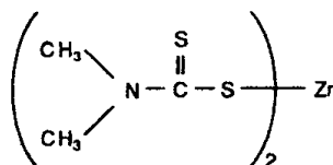
Zinc Dimethyldithiocarbamate
